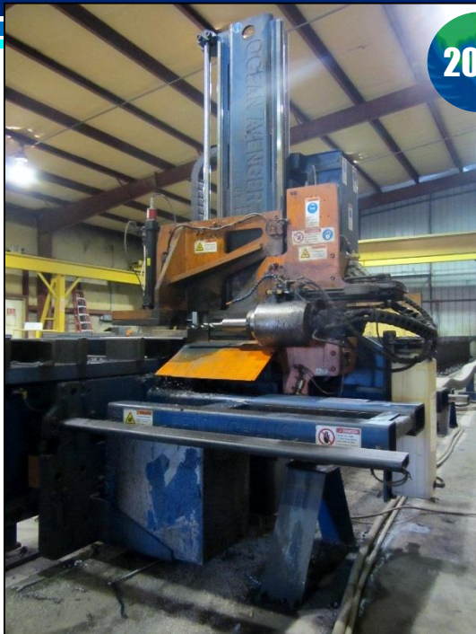
PEDDINGHAUS 1000B OCEAN AVENGER CNC BEAM DRILL
